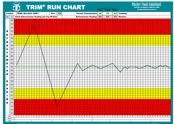
Concentration control of coolants has a direct effect on the success of coolant management programs. Every water-soluble fluid is designed to run within a specific concentration range. Fluids running below that range often have corrosion, tool and sump life problems. Running above the range often demonstrate dermatitis, residue, and excess fluid problems.
